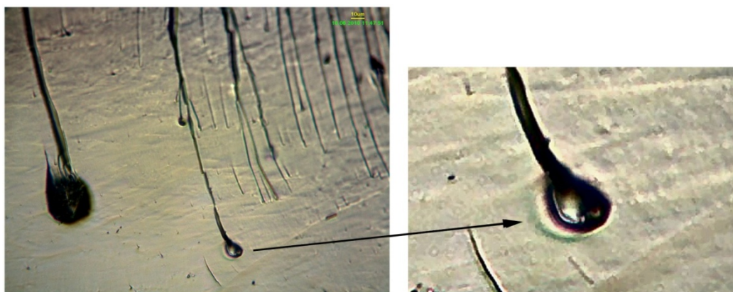
Figure 4 – Solidified fluid on the walls of "gas bubbles"
